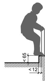
Fig. 4: Accessible (ill. bfu)
